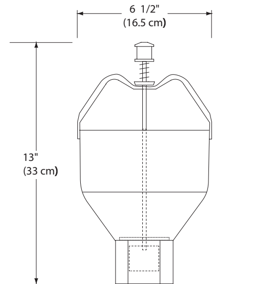
Part # K-1016WSS - Holder for Type K
