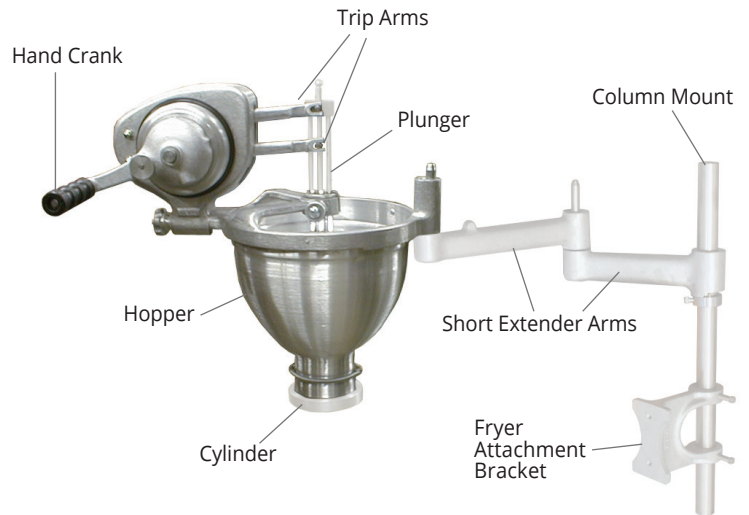
Belshaw Type N shown with column mount and short extender arms. *Mounting system, plunger and cylinder are purchased separately.
